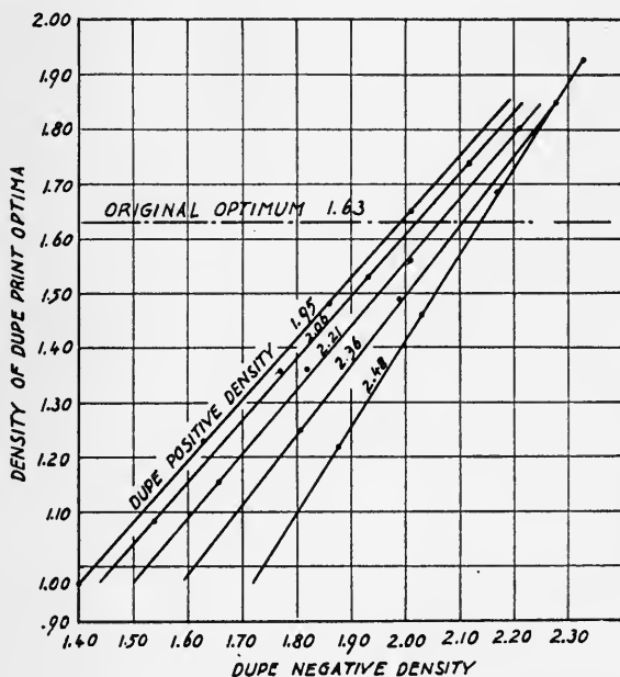
FIG. 4. Family of curves showing processing optima for a duping process using 1363 as a master positive and 1301 as a duplicate negative.
